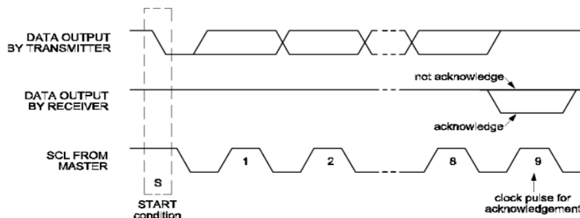
Figure 9: C bus Response
