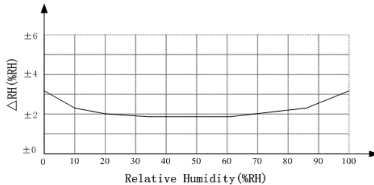
Figure 2: 25 °C relative humidity of maximum error AM2321
